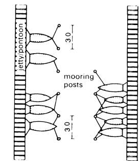
1 Berths for sport boats: in Rotterdam
